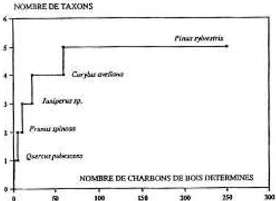
Taxonomic curve based on the gathered fragments in the fireplace F8-G8, habitat level C6 (Abeurador)
